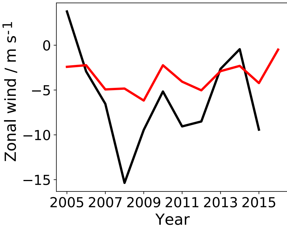
Mean summer 88 km
