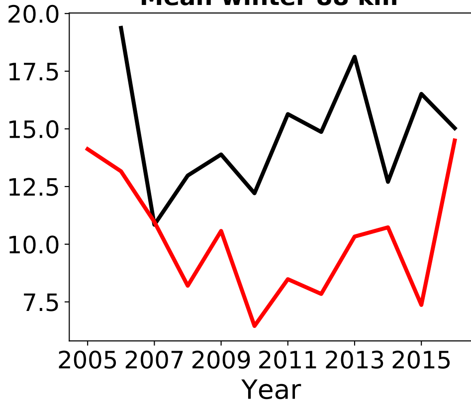
Mean winter 88 km
