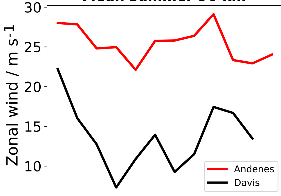
Mean summer 96 km
