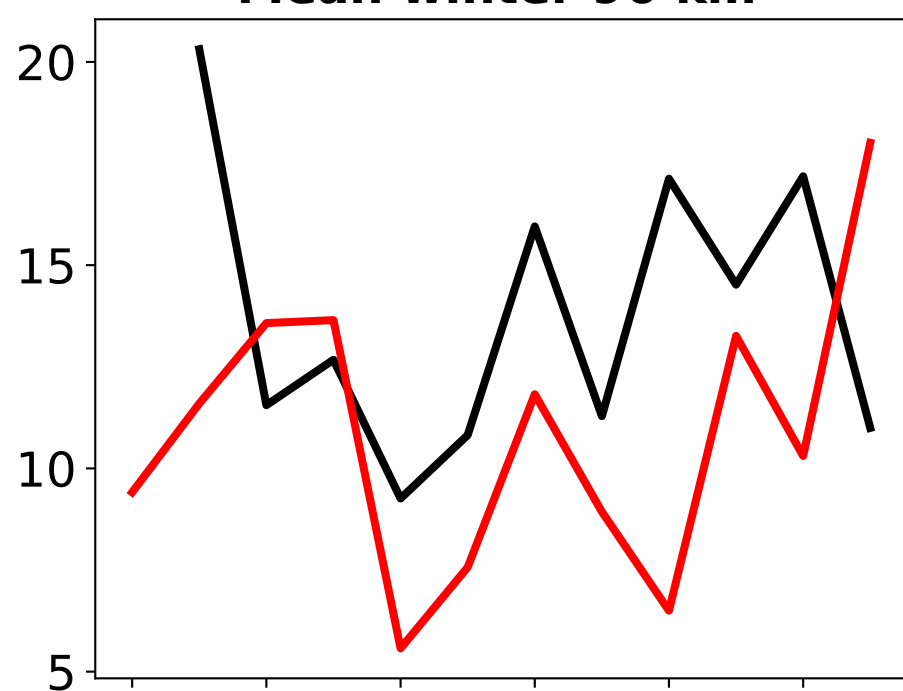
Mean winter 96 km
