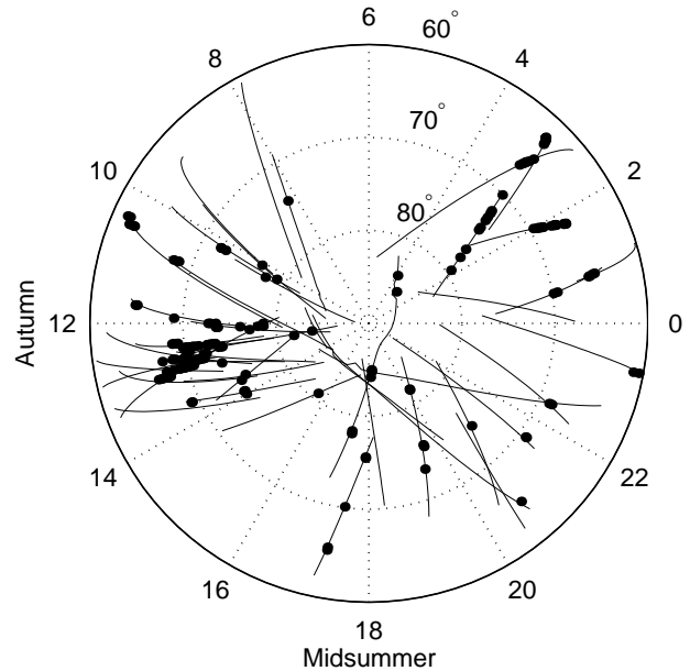
Fig. 5. Diagram with Magnetic Local Time (MLT) and invariant latitude, showing the investigated data intervals (the lines) and the location of the identified LHCs (the dots) in the Cluster data set. The total number of identified LHCs is 535, so many of the dots in the figure overlap. The altitudes of the orbits are shown in Fig. 7.
