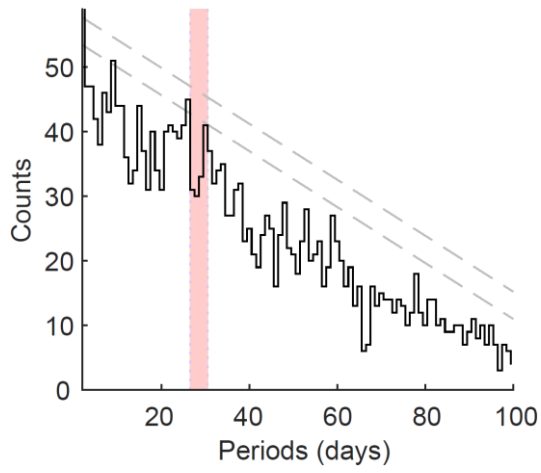
Figure S1. Periodicity of wide-area lightning activity covering more than 4 prefectures at the Sea of Japan side from November to March. The gray dashed lines correspond to 2 and 3 standard deviations. The red bars indicate the 27–30 day period.
